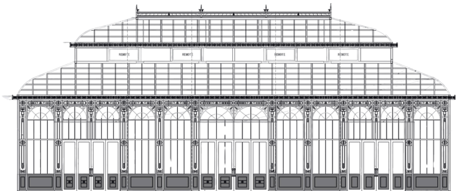
Architectural Drawing of The Conservatory at Grelen
